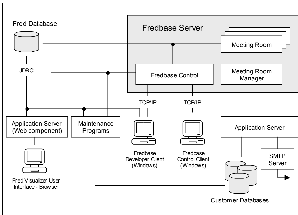
Figure 1: FredBase Architecture
